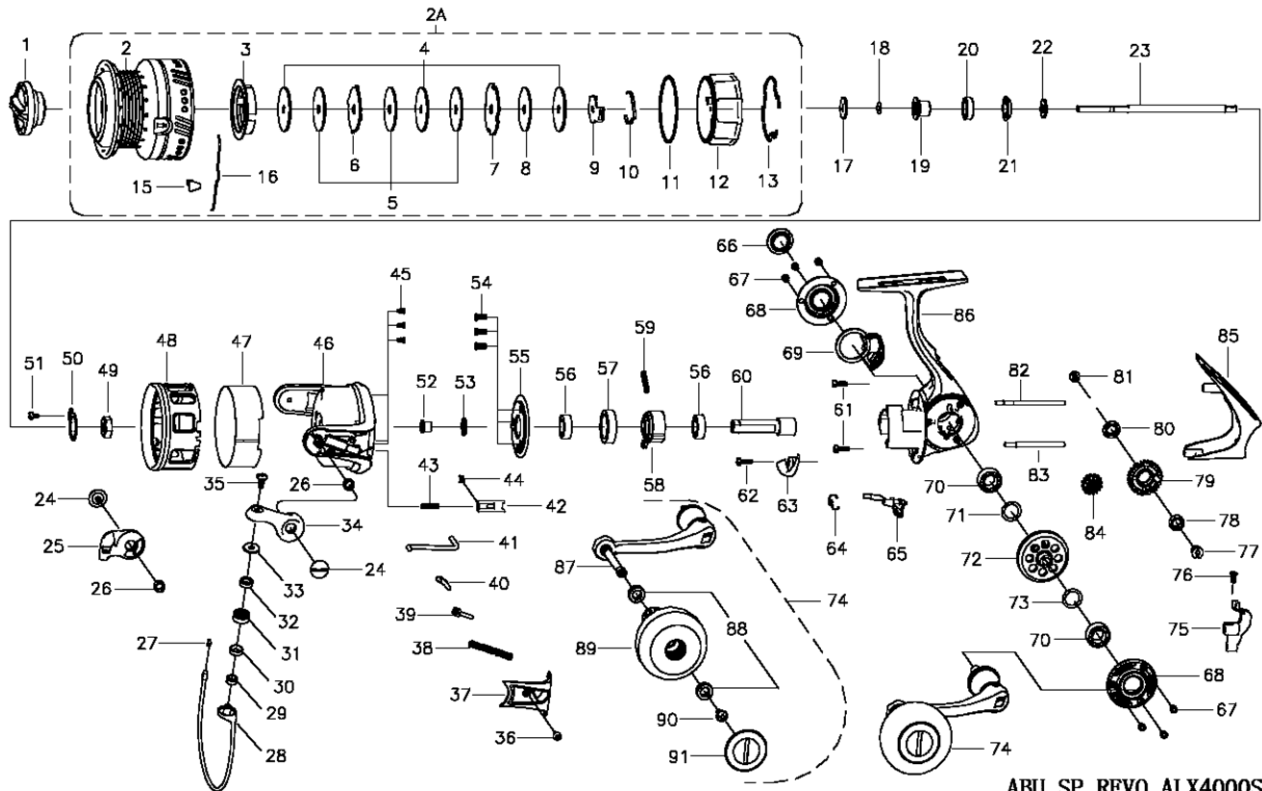
ABU SP REVO ALX4000SH 00
