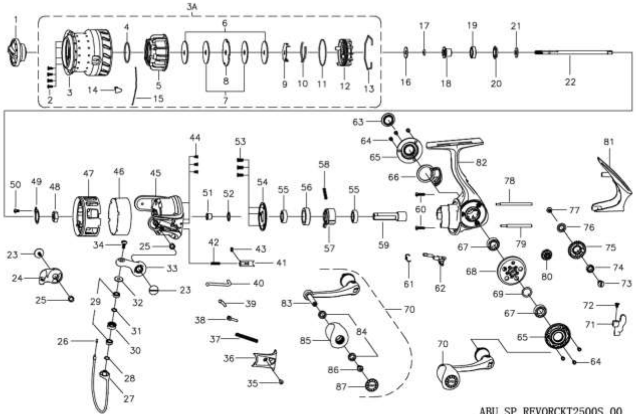
ABU SP REVO RCKT2500S 00
