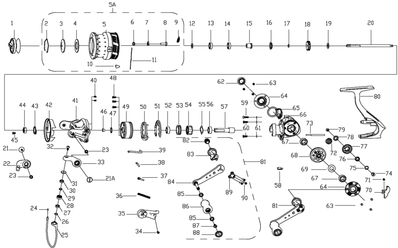
ABU SP REVO MGXTREME2500S 00
