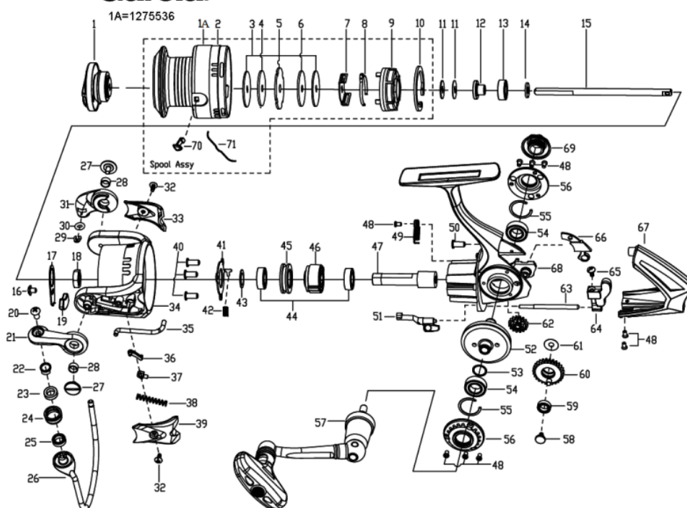
EXPLODED VIEW OF ORRA 2500S
