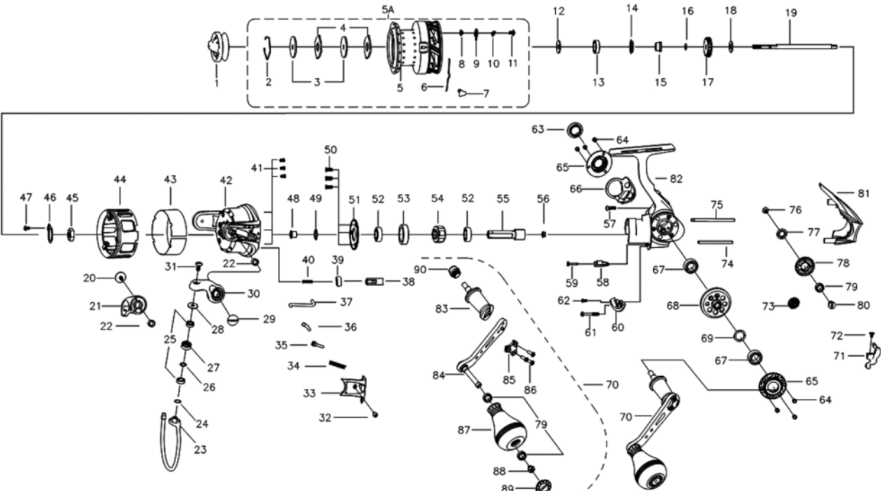
EXPLODED VIEW
