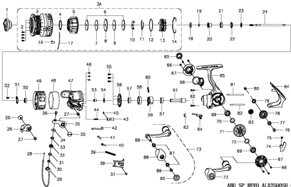
ABU SP REVO ALX2500SH 00
