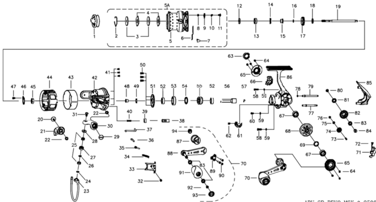
ABU SP REVO MGX θ 2500SH 00
