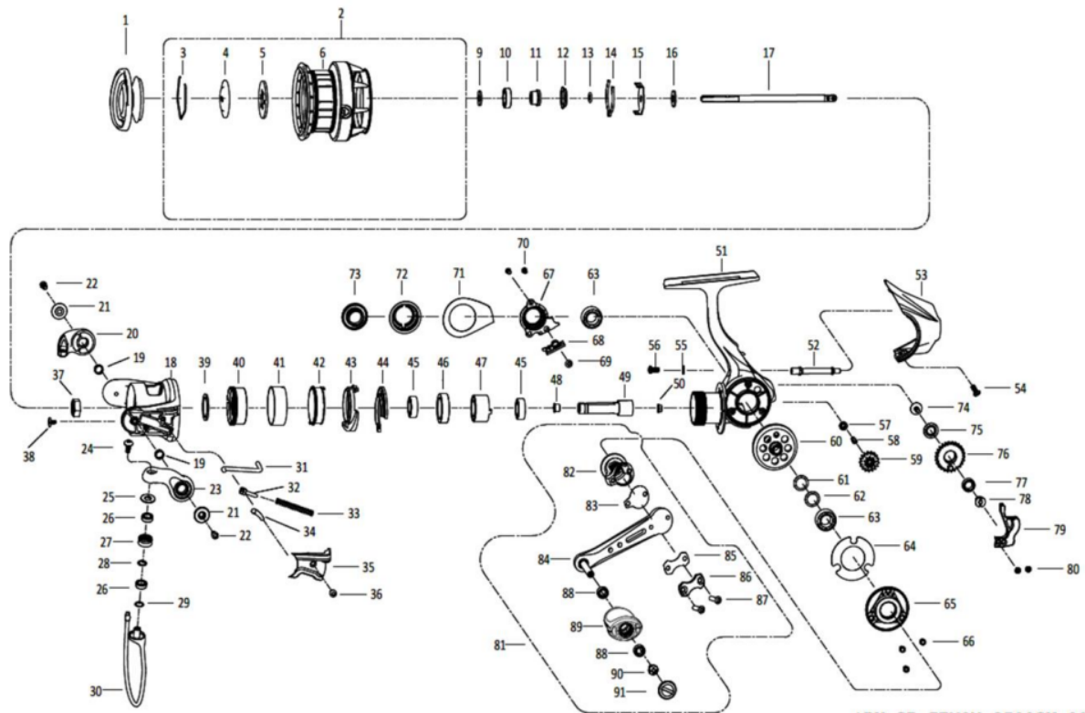
ABU SP ZENON 2500SH 00
