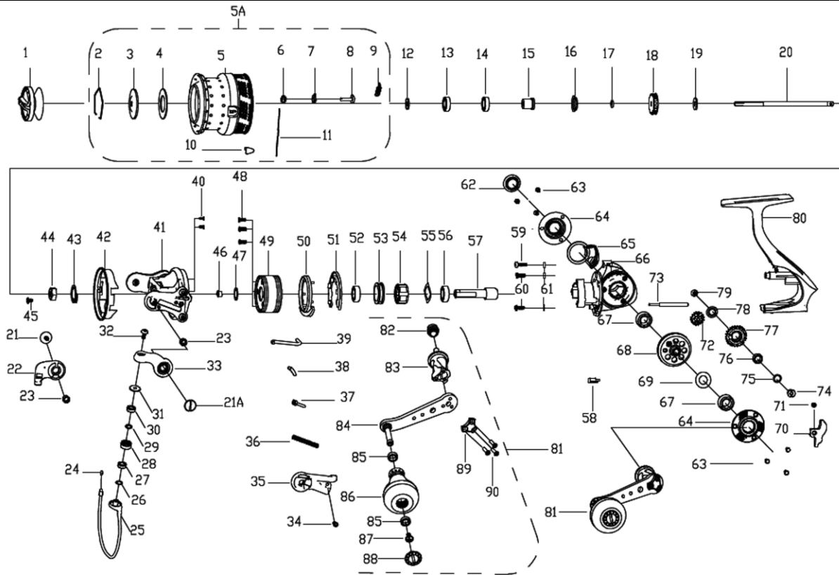
ABU REVO MGxtreme2500MSH 00
