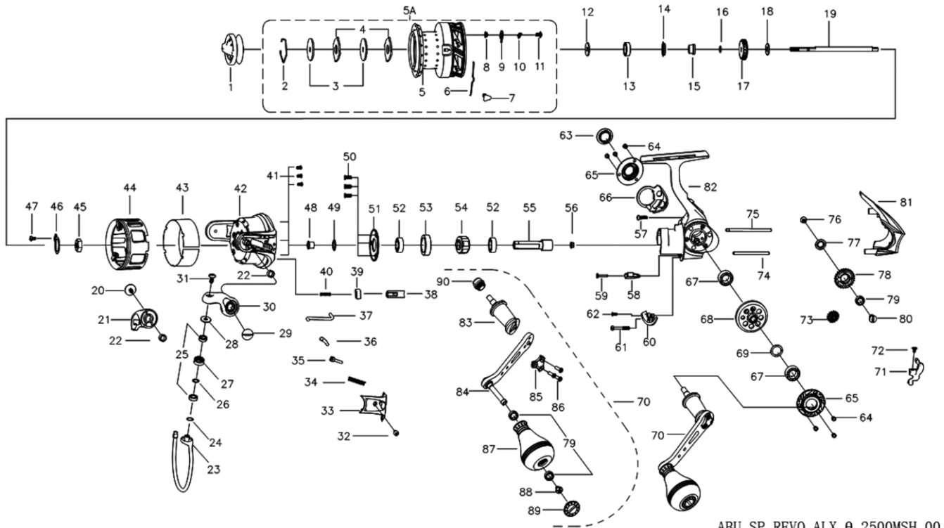
ABU SP REVO ALX θ 2500MSH 00
